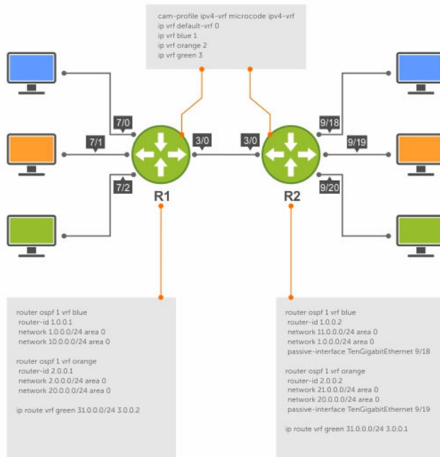
Figure 123. Setup OSPF and Static Routes
